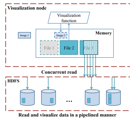
Figure 4 The process flow of visualizing time-series data files resident in HDFS. HDFS-resident data are read concurrently. Once a target file is fully aggregated, visualizing that file starts.
