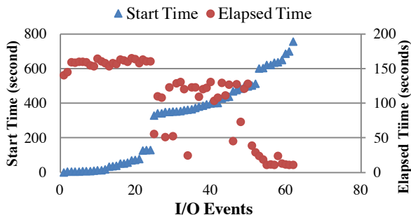
Figure 6 The performance of dynamic Hadoop reader. Data is first read directly from remote PFS and then processed with Map function of a MapReduce application (i.e., WordCount). Start time indicates the time when a read event begins. Elapsed time is the duration for a whole event.
